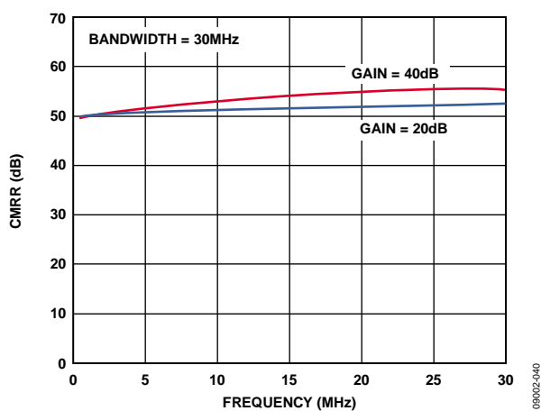
Figure 40. Common-Mode Rejection Ratio vs. Frequency (Bandwidth Setting = 30 MHz)
